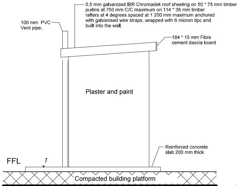
EAST ELEVATION SCALE 1: 50 on (A3)
