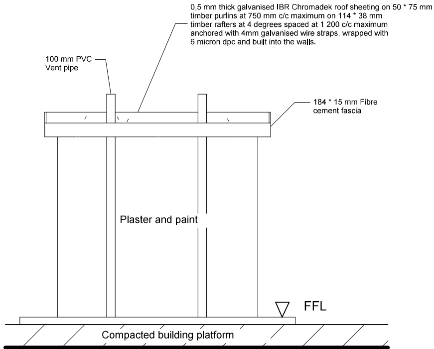
SOUTH ELEVATION SCALE 1: 50 on (A3)
