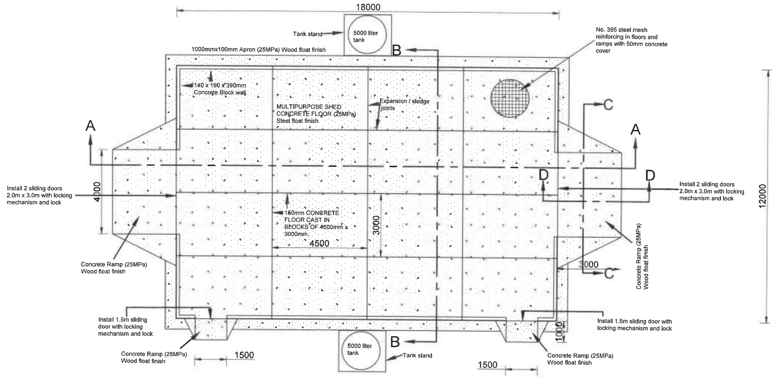
FLOOR PLAN SCALE 1 : 100 ON A3
