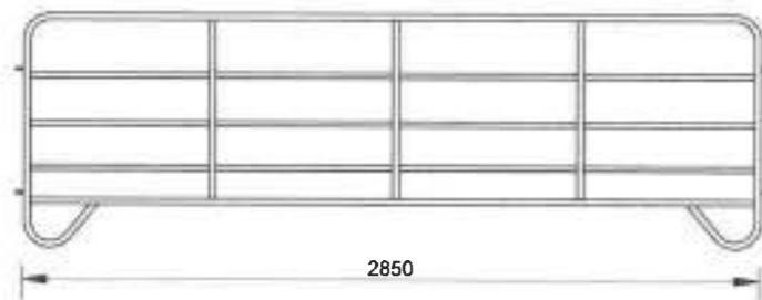
GATE SECTION 3 (GS3)
