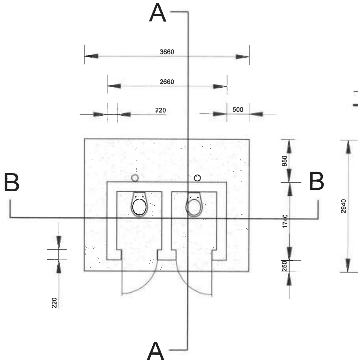
FLOOR PLAN SCALE 1: 50 on (A3)
