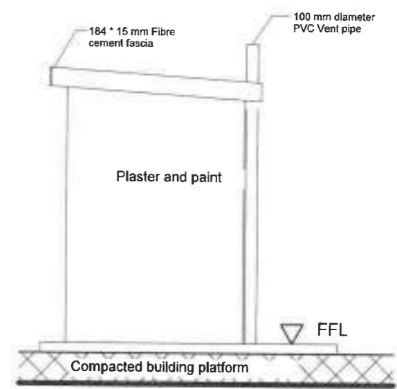
WEST ELEVATION SCALE 1: 50 on (A3)
