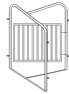
GATE SECTION 7 (GS7)
