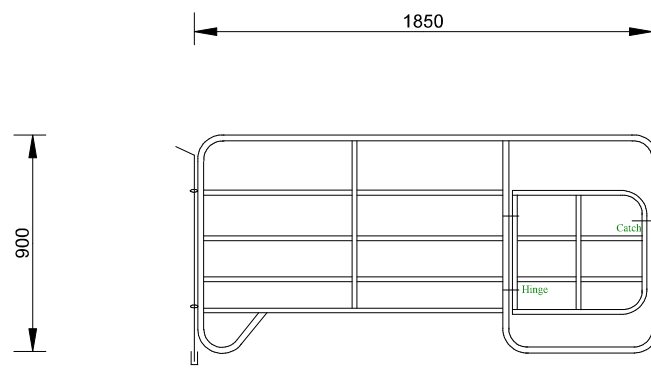
GATE SECTION 1 (GS1)
