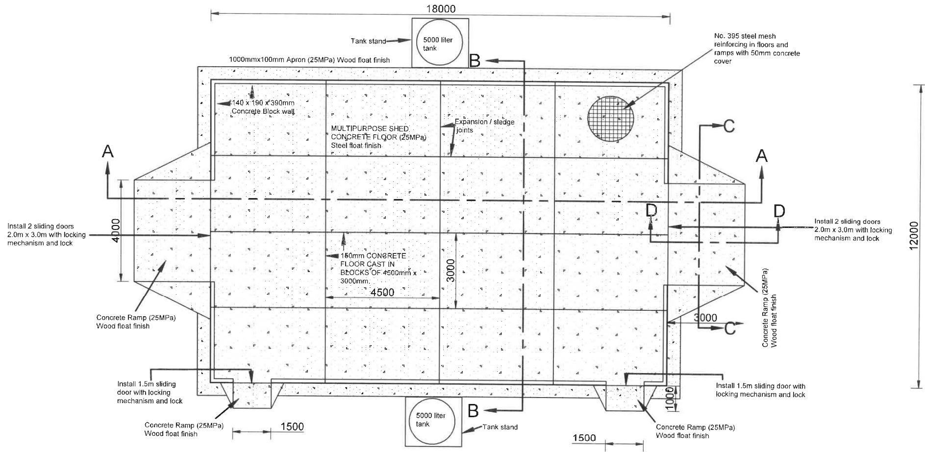
FLOOR PLAN SCALE 1 : 100 ON A3
