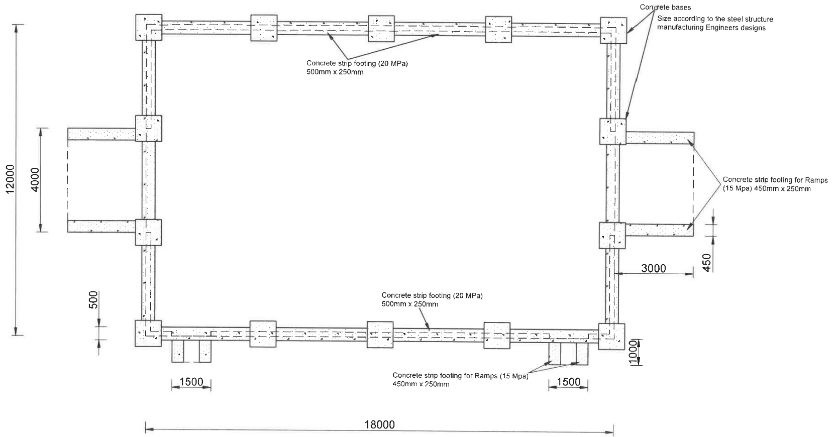
FOUNDATION PLAN SCALE 1 : 100 ON A3
