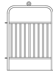
Premanufactured Guillotine gate (Taltec TSK 4 or similar)
