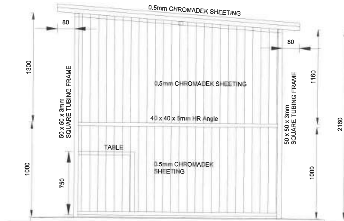
SIDE ELEVATION
