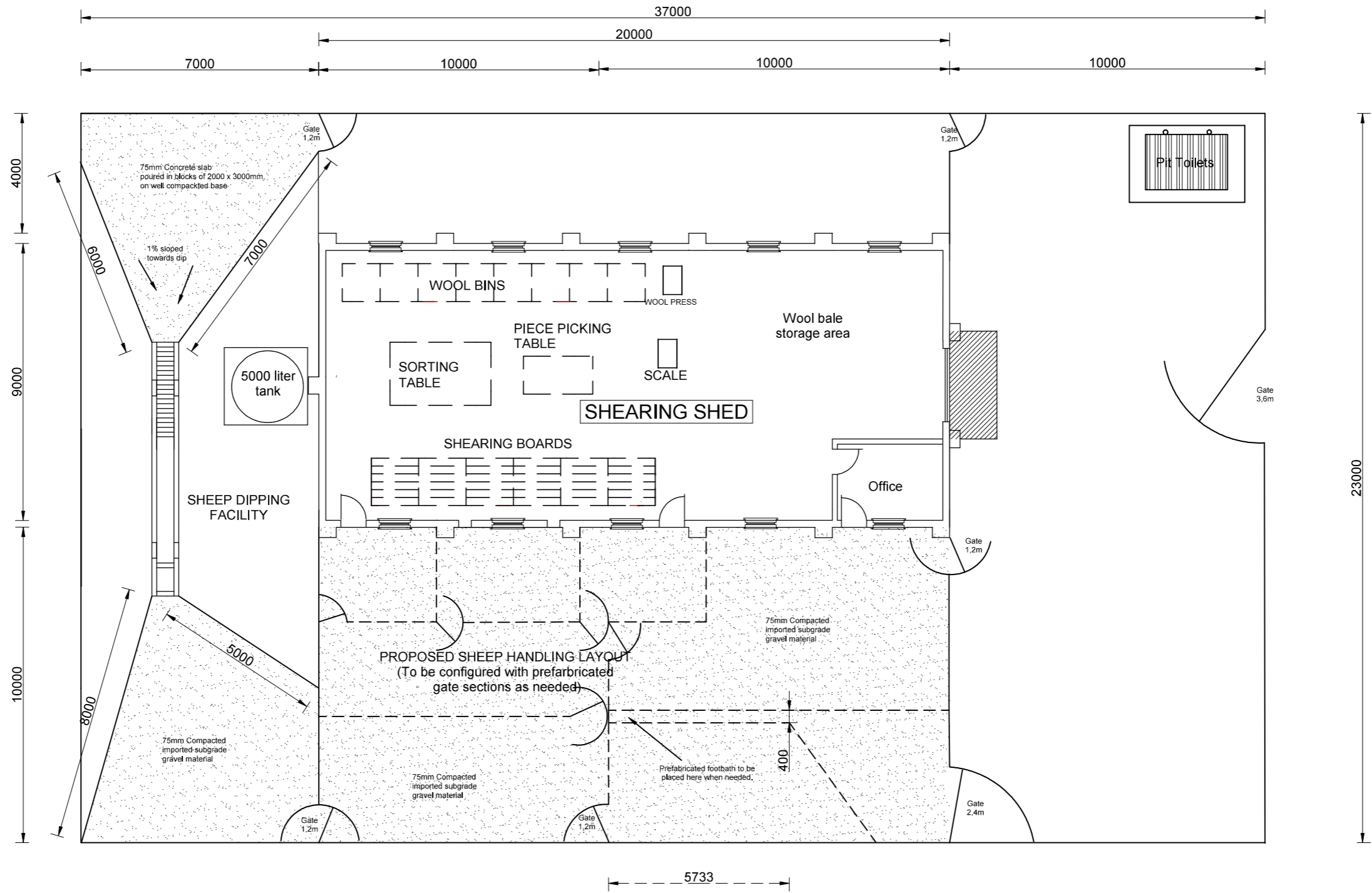
SITE LAYOUT SCALE 1:150
