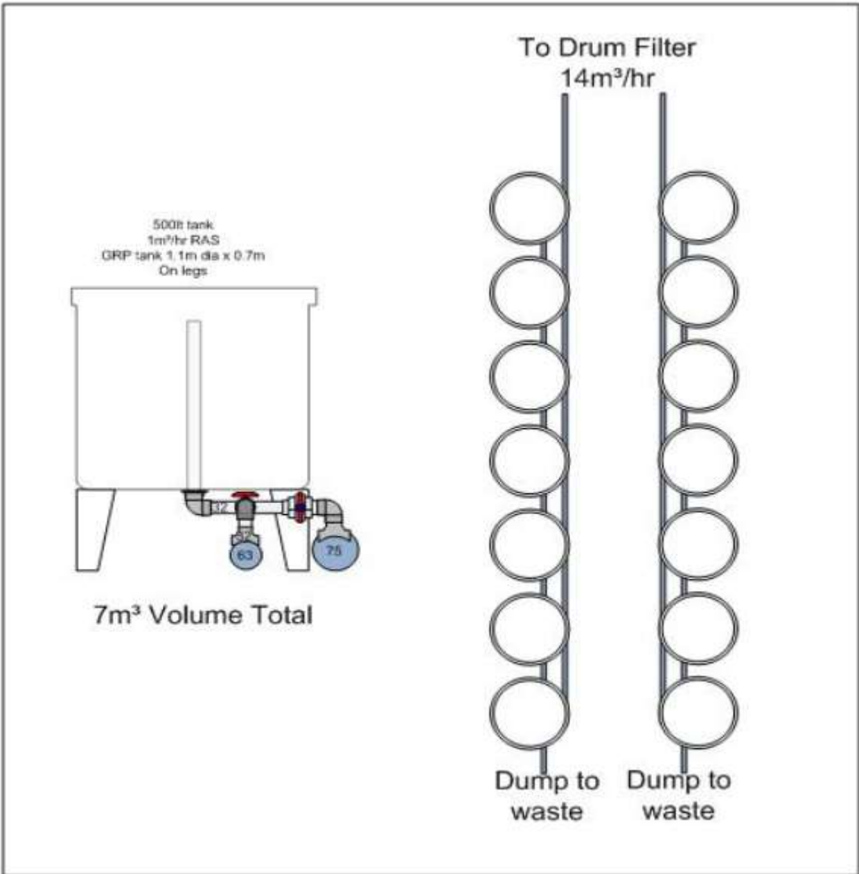
Figure 5. Juvenile Facility constructed from 500lt fibreglass tanks
