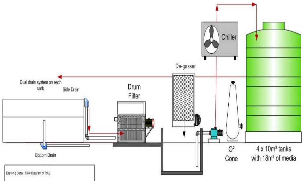
Figure 1. RAS and Flow Diagram of the system.
